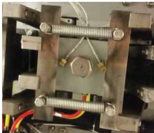
New N8 top squeezer springs
